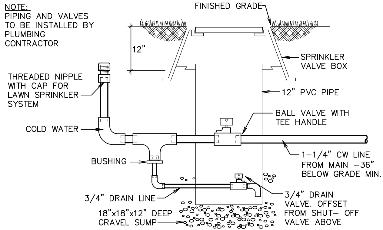
A LAWN IRRIGATION STOP & WASTE VALVE ASSEMBLY DETAIL SCALE: NONE
