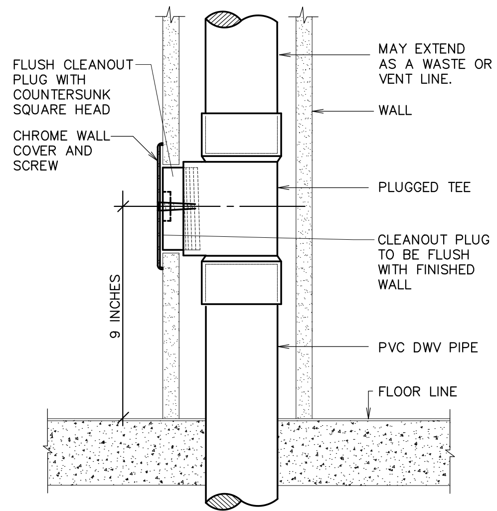
D WALL CLEANOUT DETAIL SCALE: NONE
