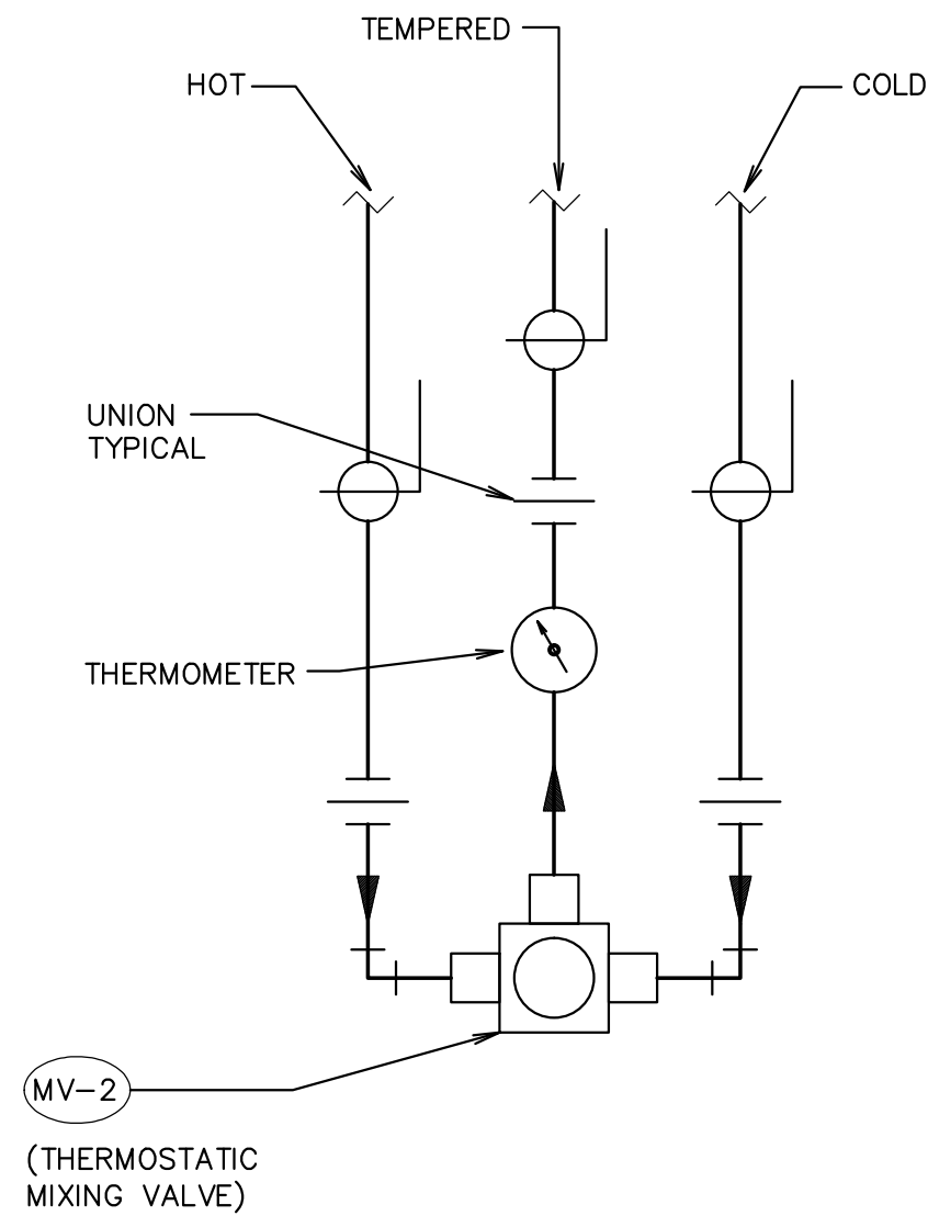
C MIXING VALVE PIPING SCHEME SCALE: NONE
