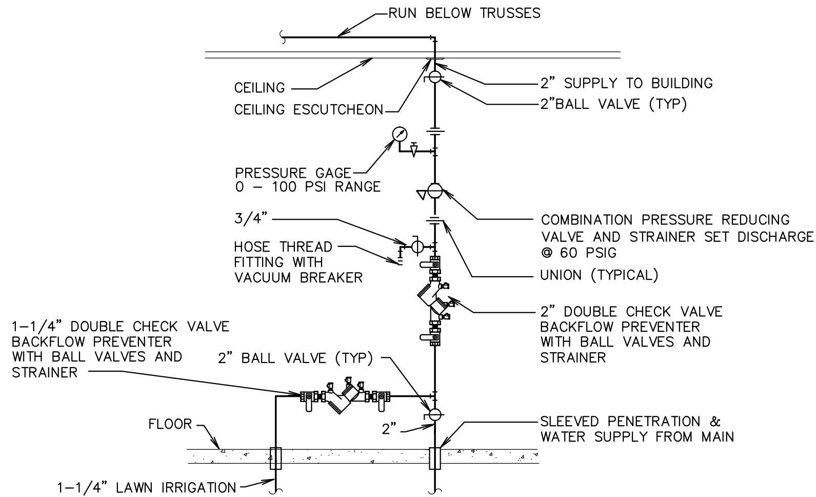
B VERTICAL WATER PRESSURE REDUCING STATION DETAIL SCALE: NONE
