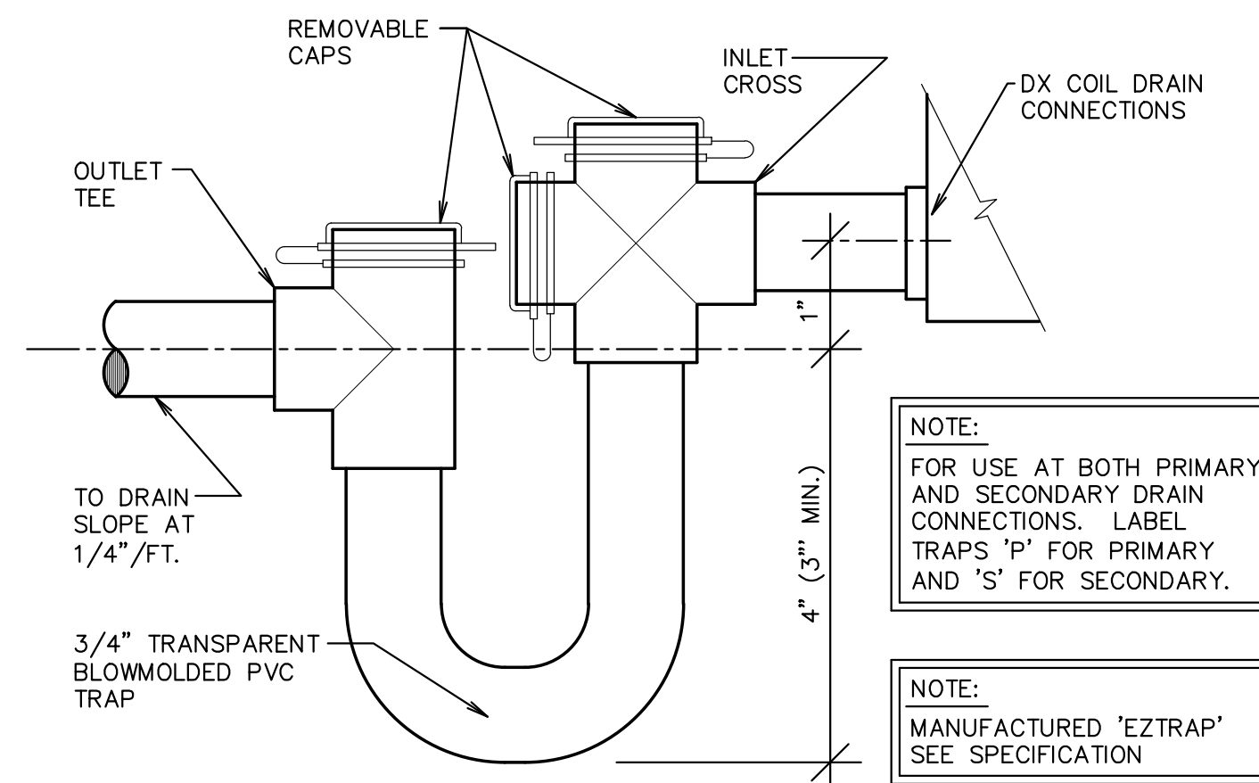
K DX COIL CONDENSATE DRAIN DETAIL SCALE: NONE
