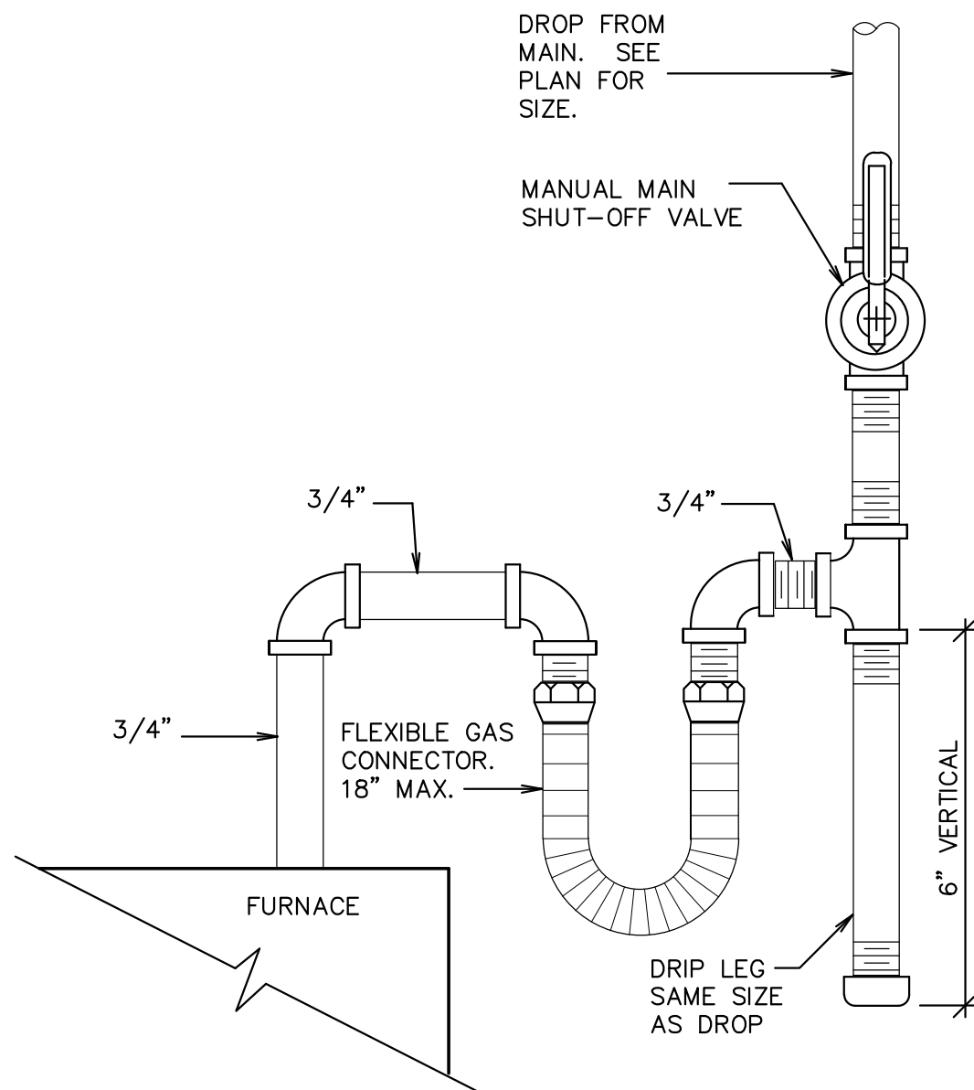
J GAS LINE CONNECTION DETAIL SCALE: NONE
