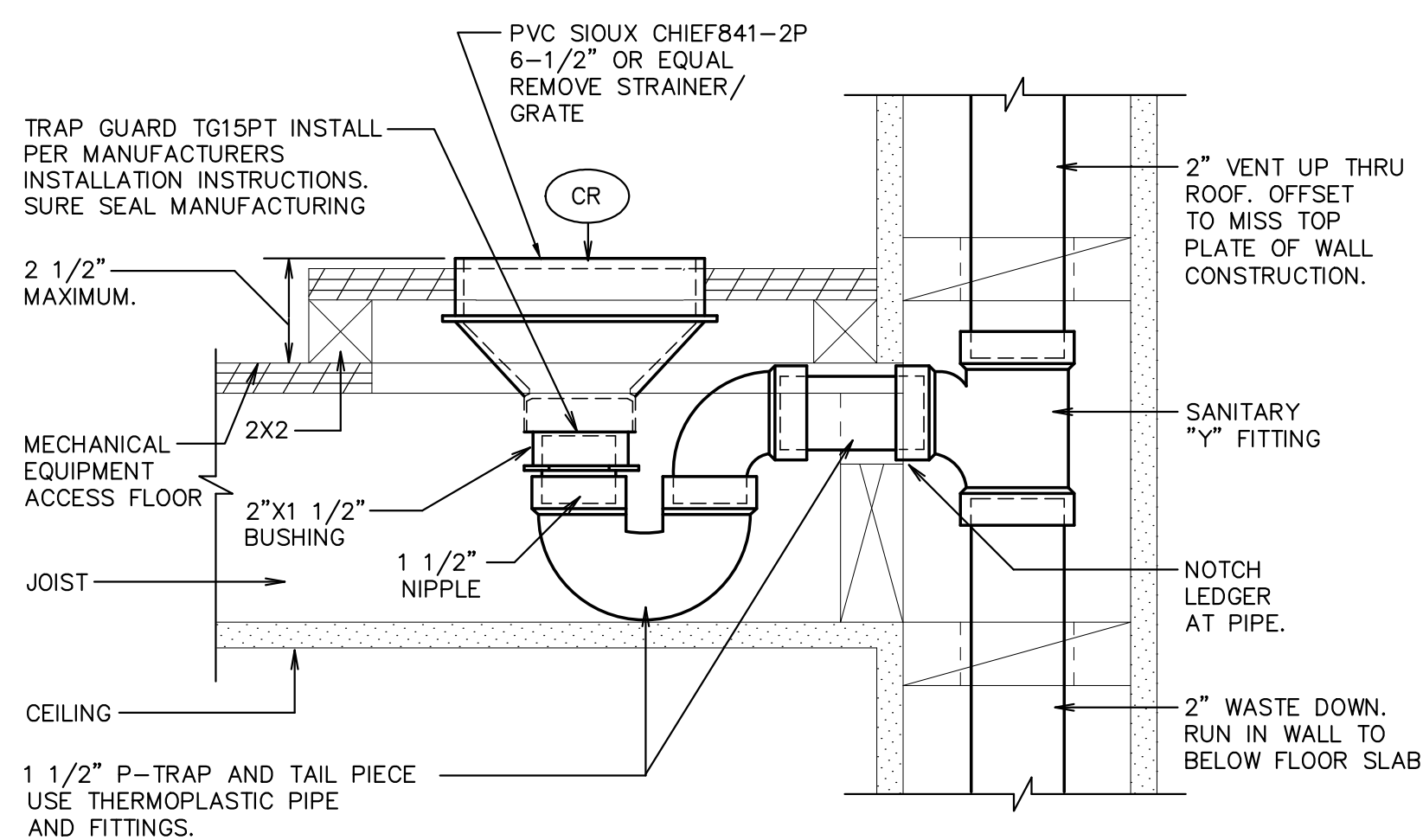
H CONDENSATE RECEIVER DETAIL SCALE: NONE
